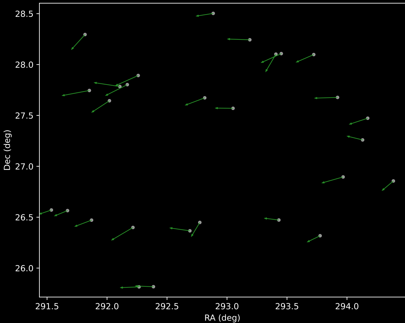
APOGEE DR17 Cluster 4 Proper Motion Vectors (n=28)
