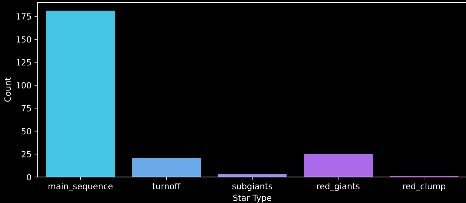
APOGEE DR17 Field: [NGP] Count plot of Star Type
