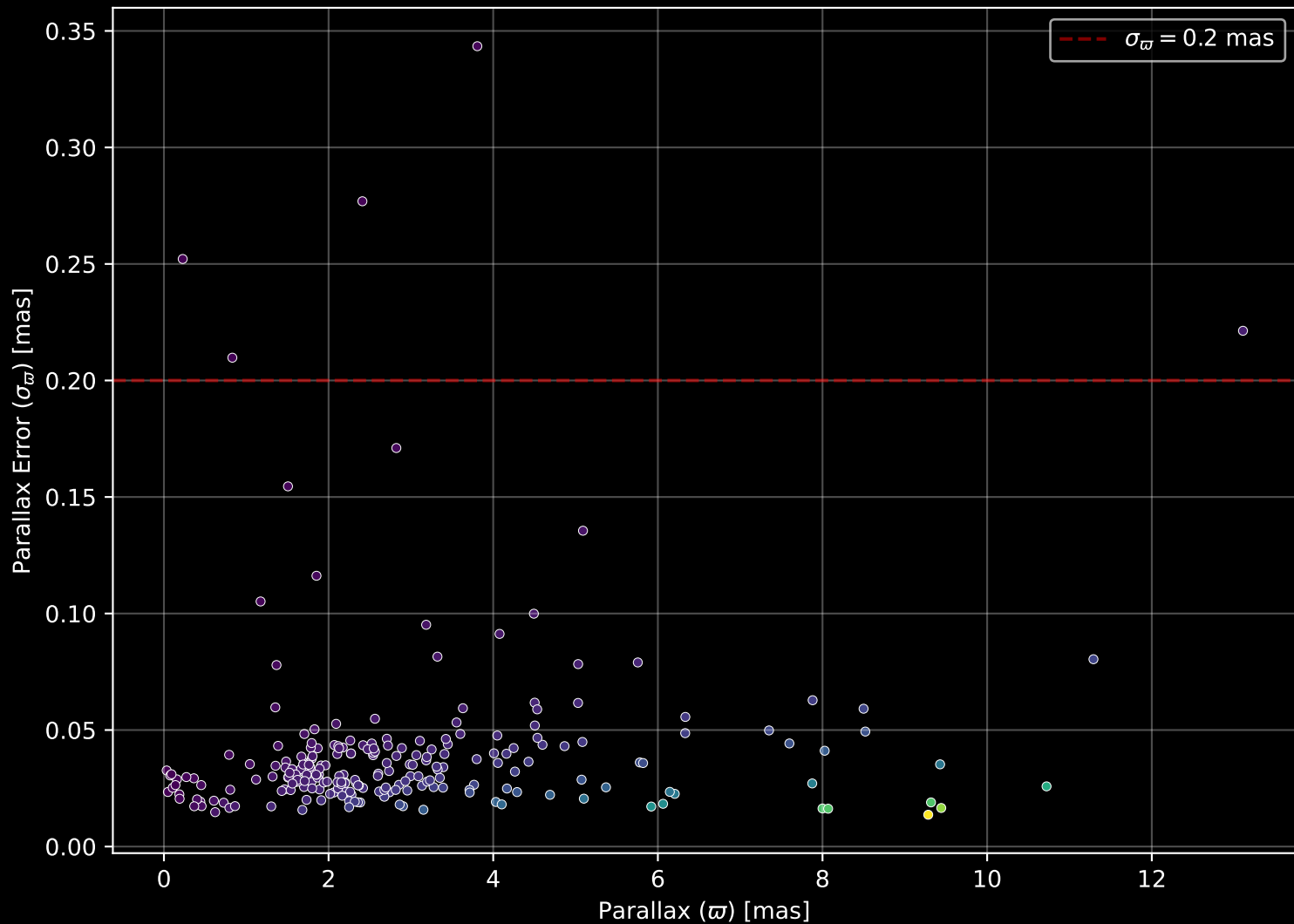
APOGEE DR17 Field: [NGP] Parallax Quality (n= 231)
