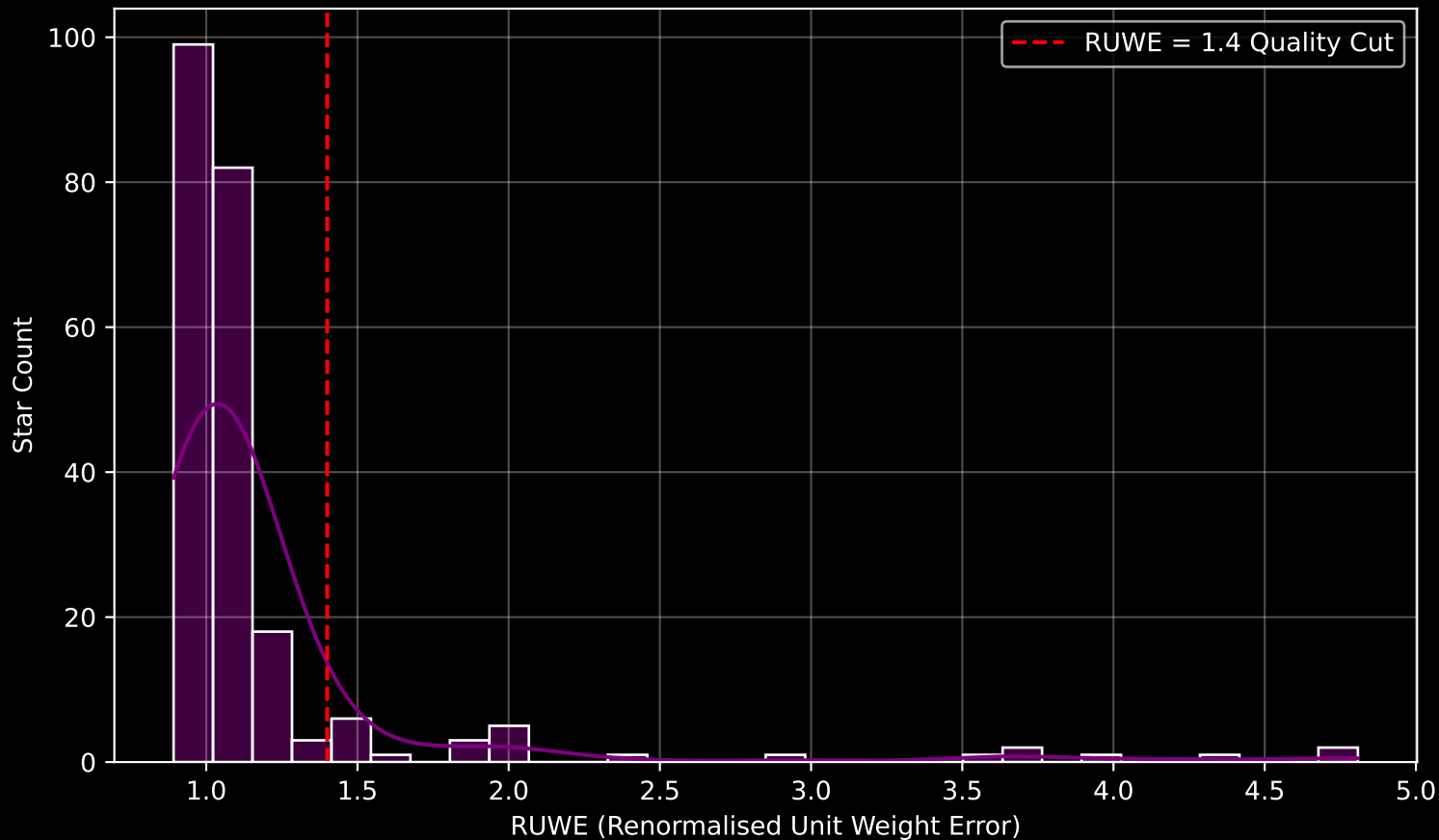
GAPOGEE DR17 Field [NGP] RUWE Distribution (n= 226)
