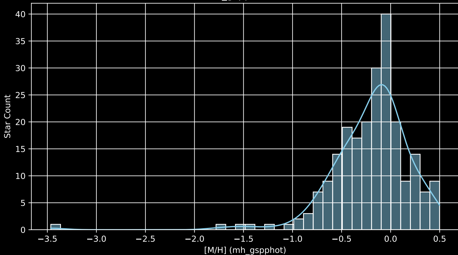
APOGEE DR17 Field: [NGP [M/H] (mh_gspphot) (n= 226)
