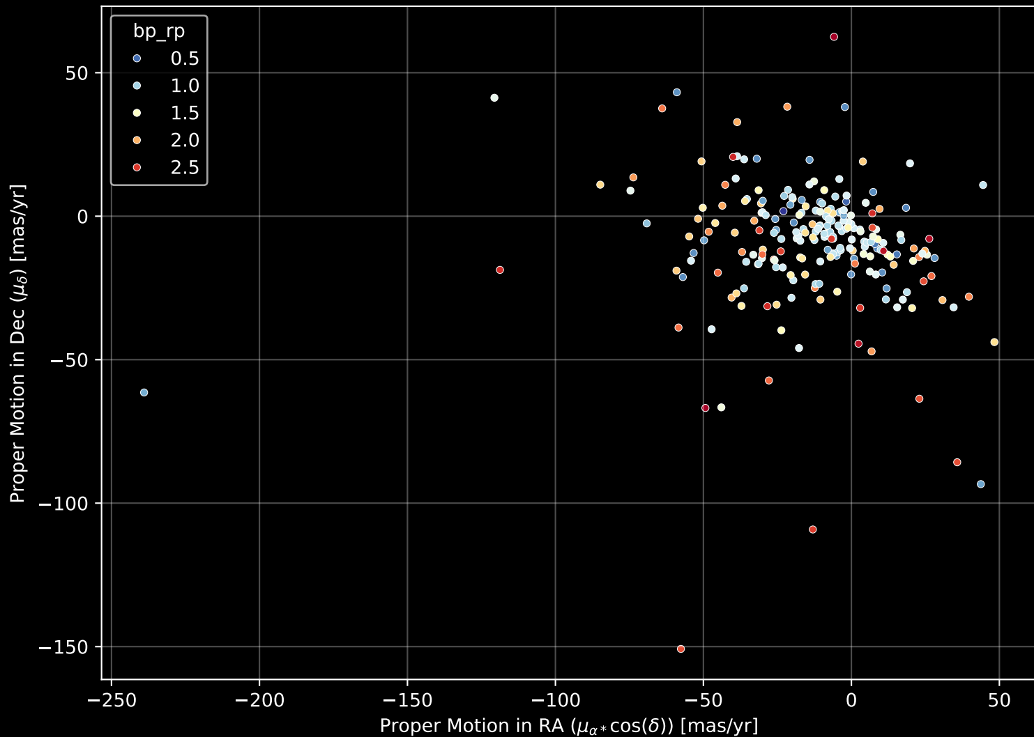
APOGEE DR17 Field: [NGP] Proper Motion Diagram (n= 231)
