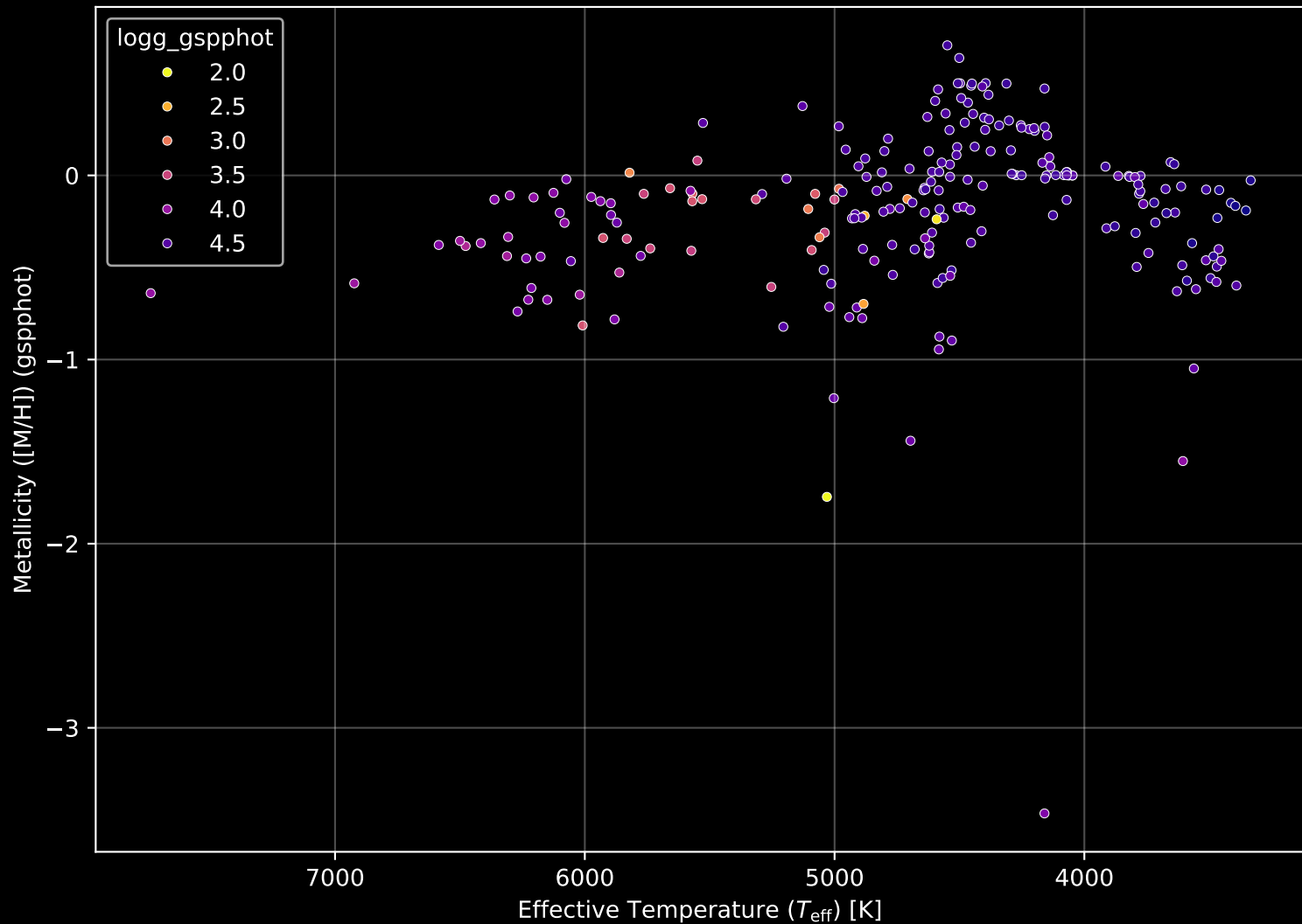
APOGEE DR17 Field: [NGP] Stellar Population Parameters (n= 231)
