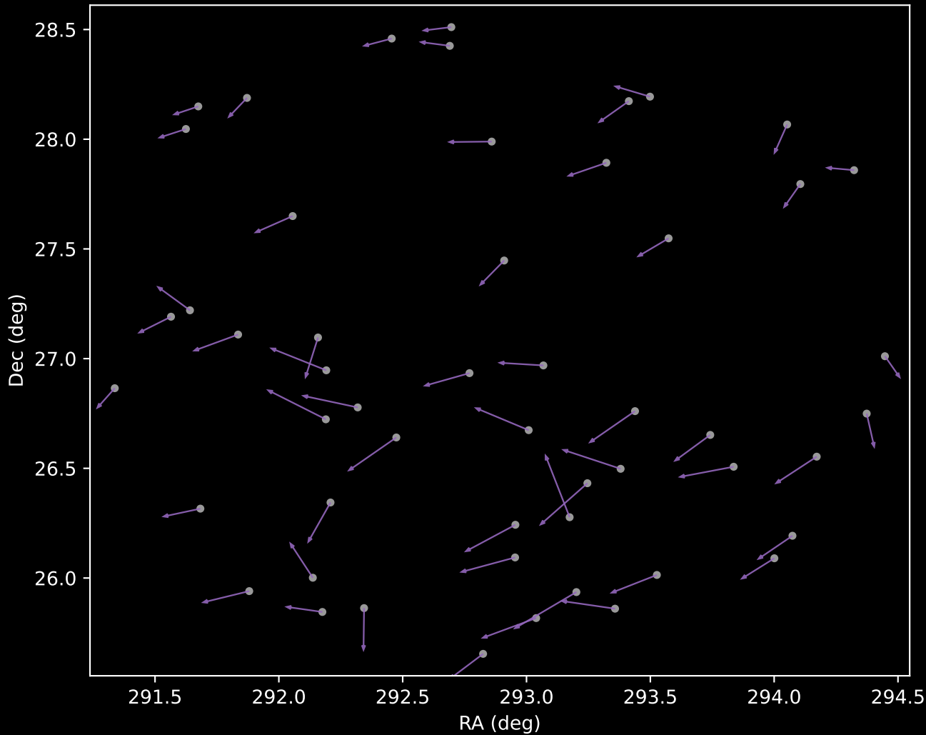
APOGEE DR17 Cluster 8 Proper Motion Vectors (n=52)
